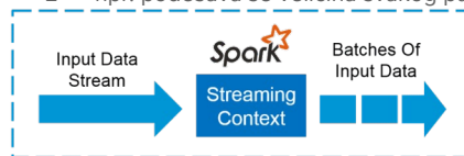
Figure: Spark Streaming Context
