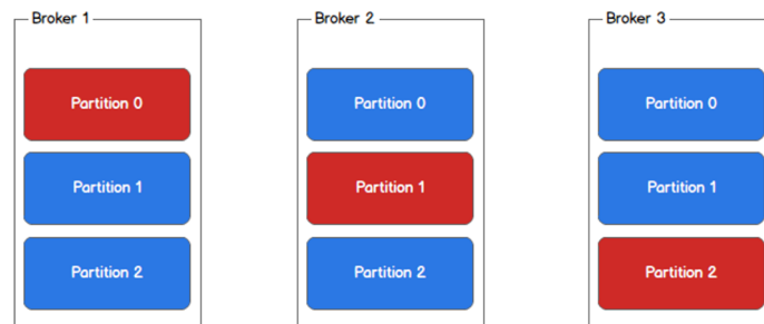
Leader (red) and replicas (blue)
